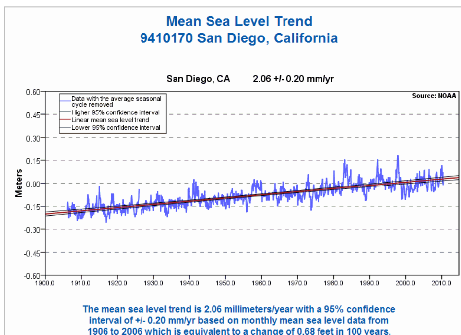
Figure 3.4. The relative mean sea level trend for San Diego, CA
